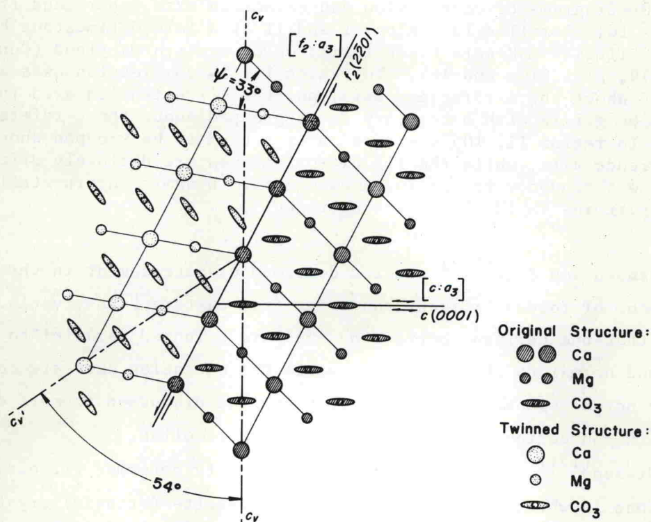
Fig. 31—Diagrammatic representation of the dolomite structure. Plane of the section is parallel to a_3(11\bar{2}0) . Gliding direction for translation on \{0001\} is not in the plane of the section, but is parallel to any of the three a axes. The system for twin gliding parallel to f is also illustrated.
