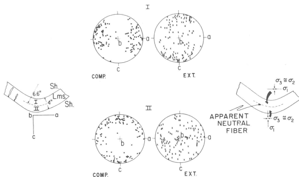
Fig. 30—Diagrams of compression and extension axes determined from calcite twin lamellae in regions I and II of a folded limestone bed in the Silurian McKenzie Creek formation of western Maryland (Conel, Ref. 119, Figs. 10a and 14). In region I, 114 compression axes are grouped about the a reference axis, and the 117 extension axes form a wide bc girdle with a tendency to be grouped about the c reference axis. In region II, 105 compression axes tend to be grouped about the c reference axis, while the 112 extension axes are diffusely oriented but show a tendency to lie in an ab girdle. Dynamic interpretation of these patterns is idealized at the right.
